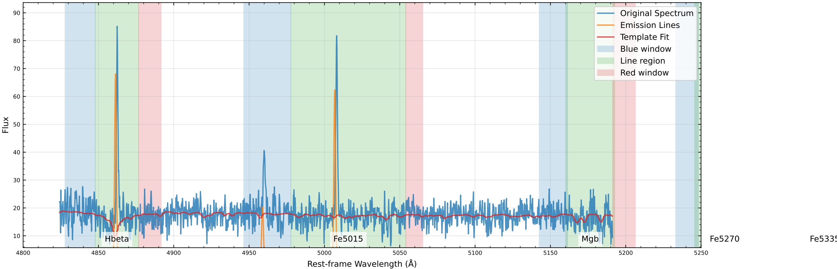
Original Data Comparison (v_star=49.4 km/s, v_gas=72.7 km/s)
