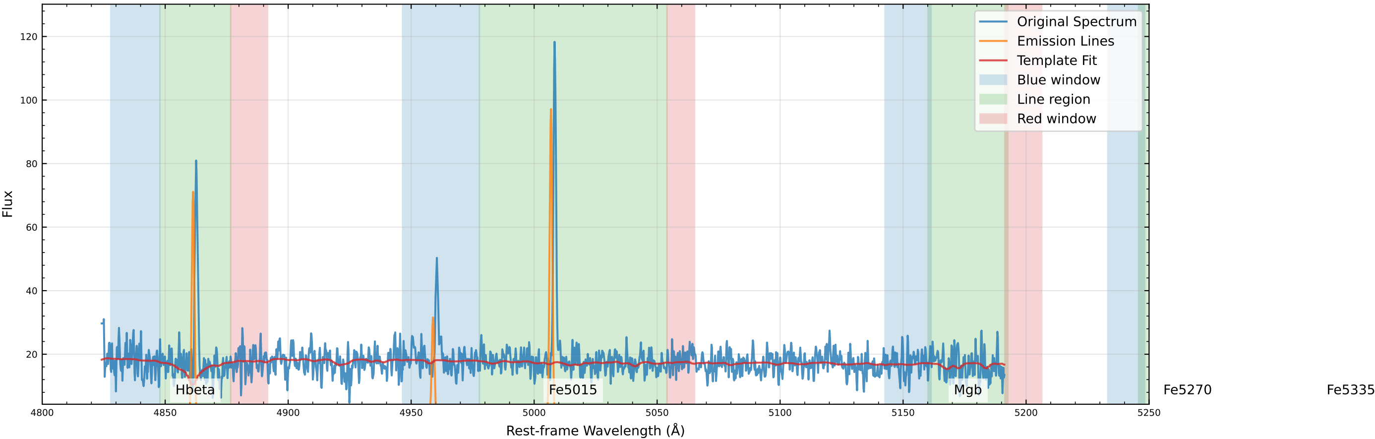
Original Data Comparison (v_star=80.0 km/s, v_gas=88.9 km/s)
