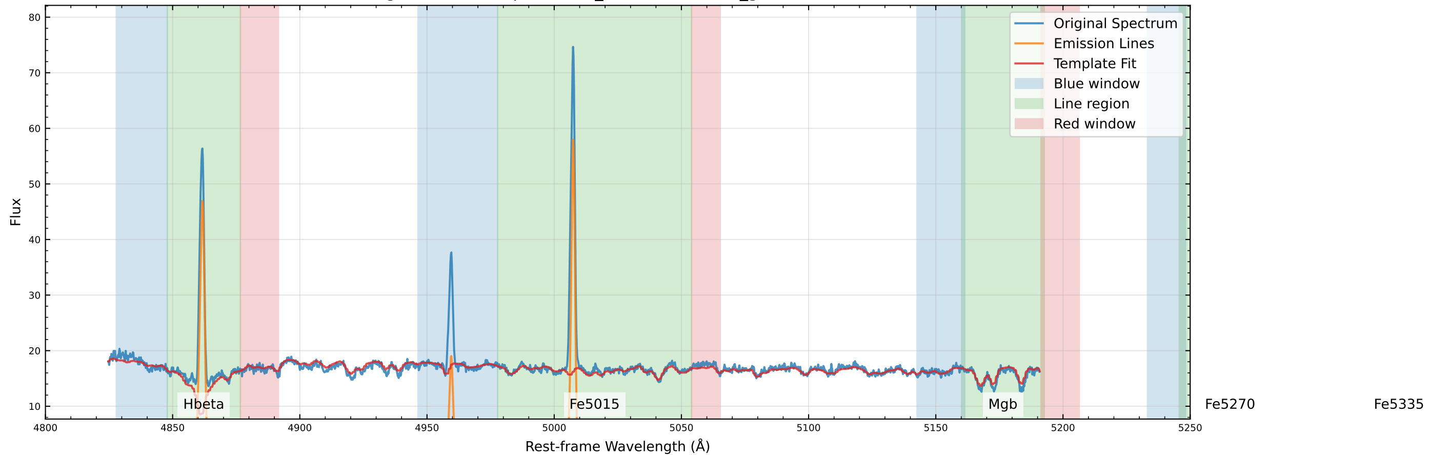
Original Data Comparison (v_star=9.8 km/s, v_gas=-7.5 km/s)
