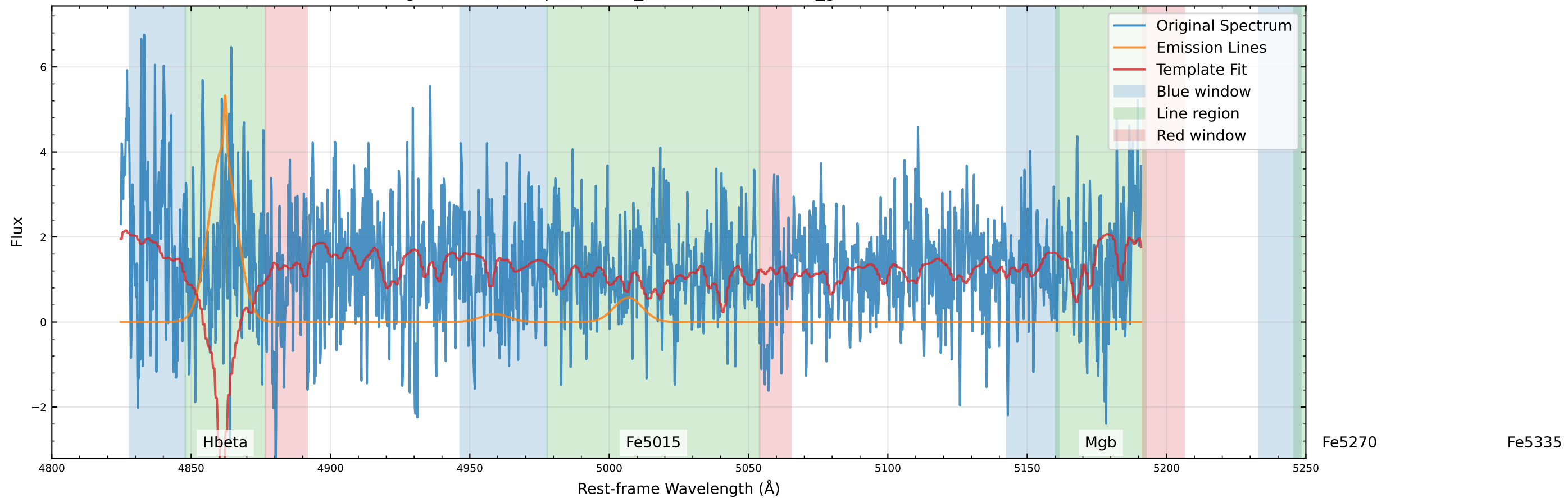
Original Data Comparison (v_star=488.9 km/s, v_gas=427.6 km/s)
