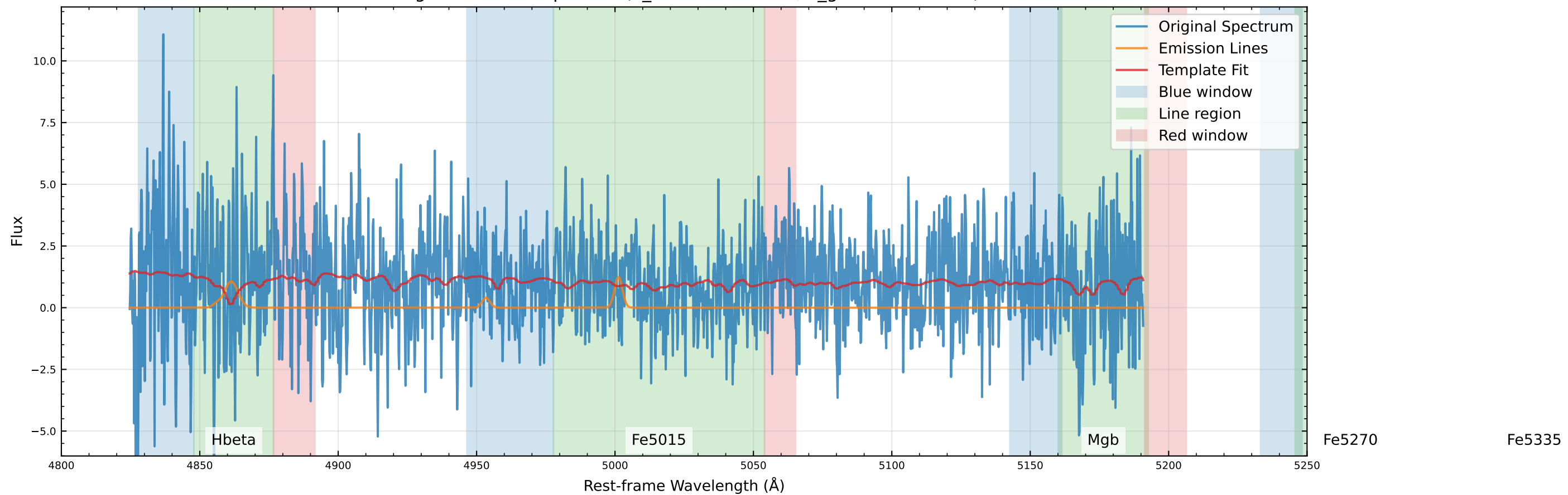
Original Data Comparison (v_star=-23.1 km/s, v_gas=276.9 km/s)
