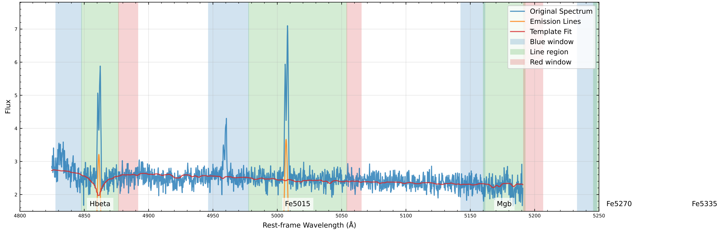
Original Data Comparison (v_star=-30.5 km/s, v_gas=28.4 km/s)
