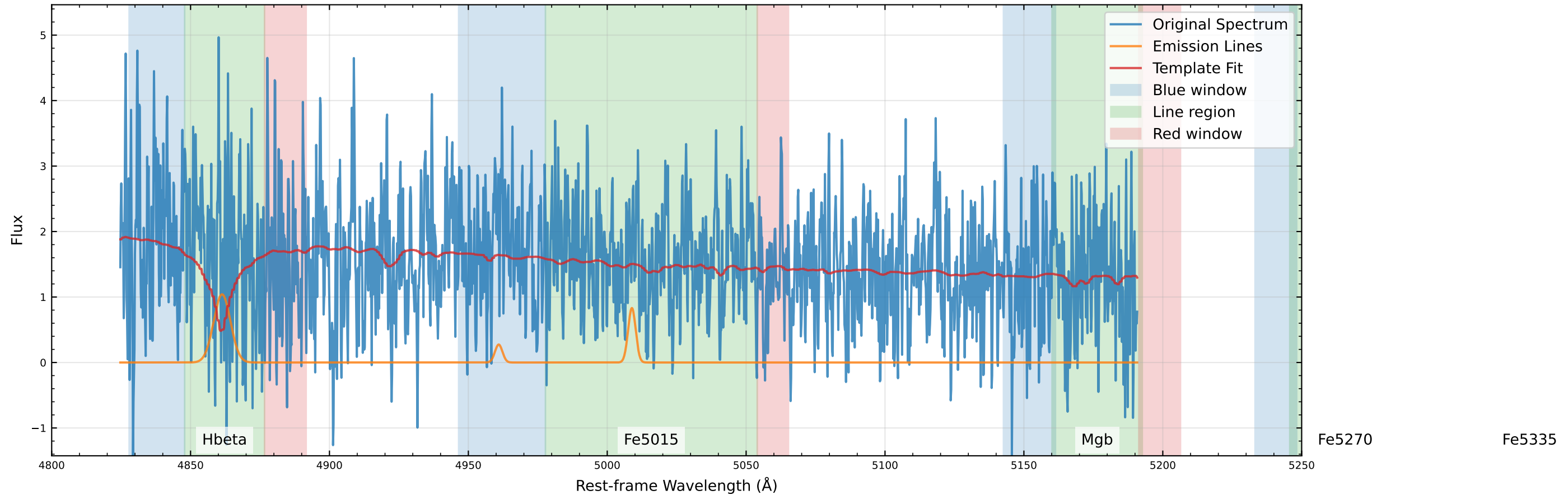
Original Data Comparison (v_star=60.2 km/s, v_gas=38.7 km/s)
