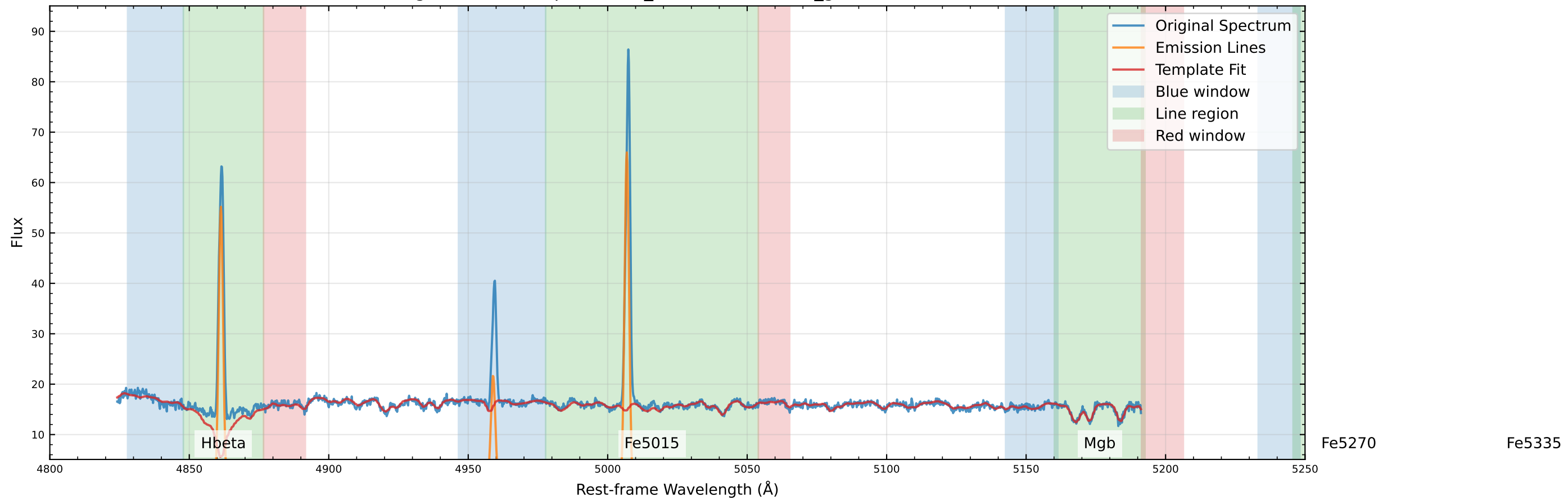
Original Data Comparison (v_star=11.3 km/s, v_gas=20.2 km/s)
