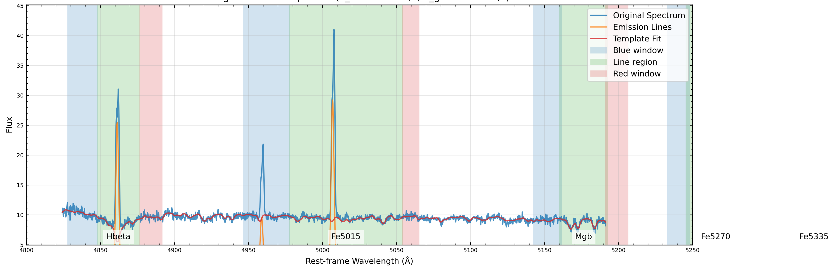
Original Data Comparison (v_star=9.7 km/s, v_gas=26.5 km/s)
