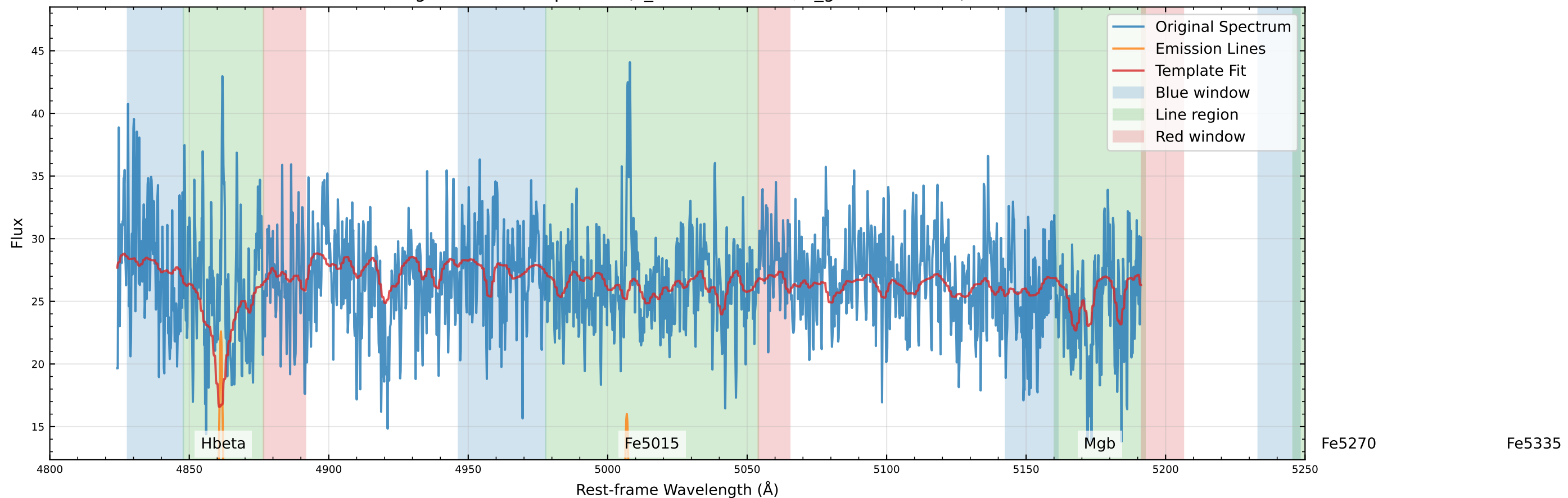
Original Data Comparison (v_star=26.3 km/s, v_gas=41.0 km/s)
