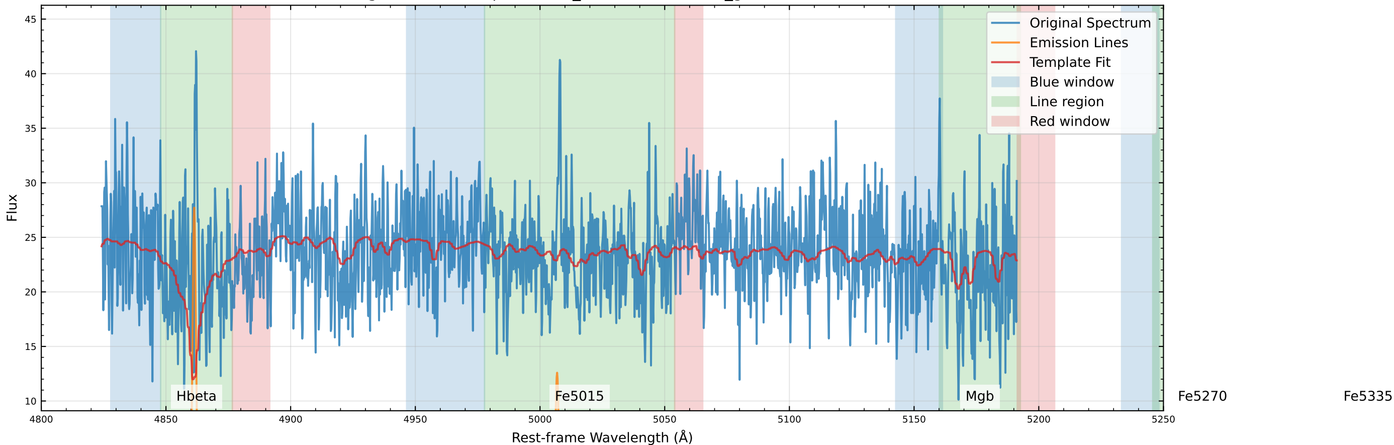
Original Data Comparison (v_star=40.8 km/s, v_gas=47.4 km/s)
