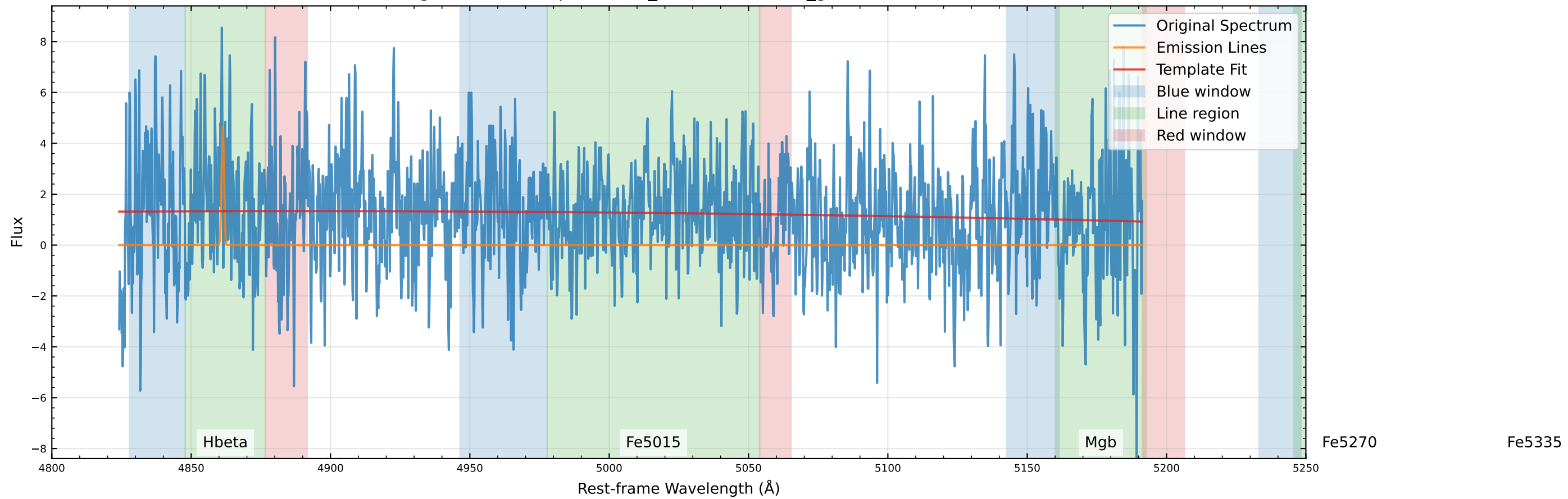
Original Data Comparison (v_star=0.0 km/s, v_gas=-30.6 km/s)
