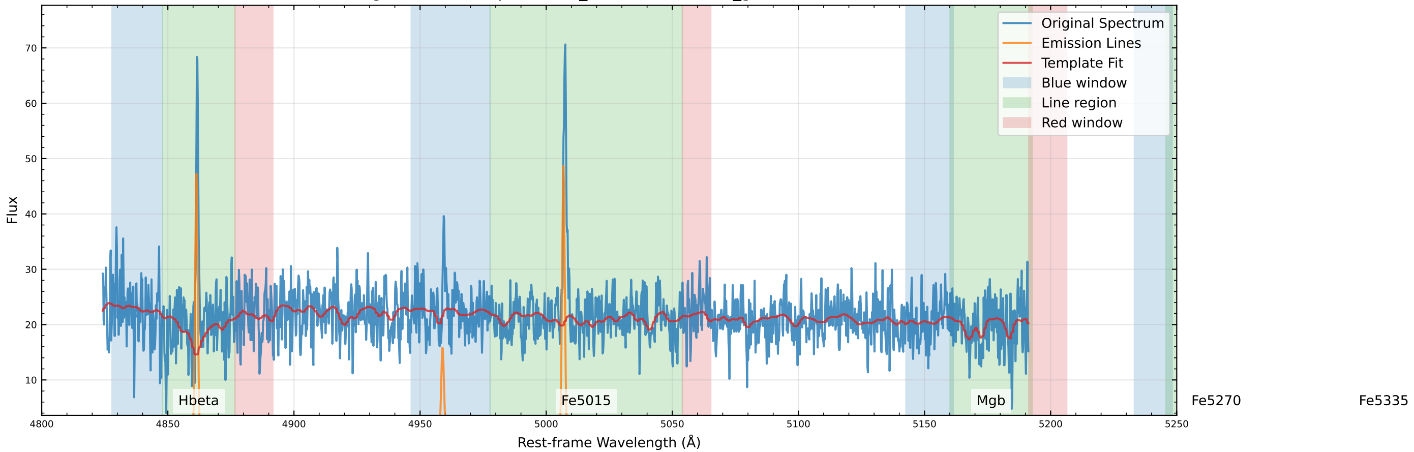
Original Data Comparison (v_star=21.0 km/s, v_gas=27.4 km/s)
