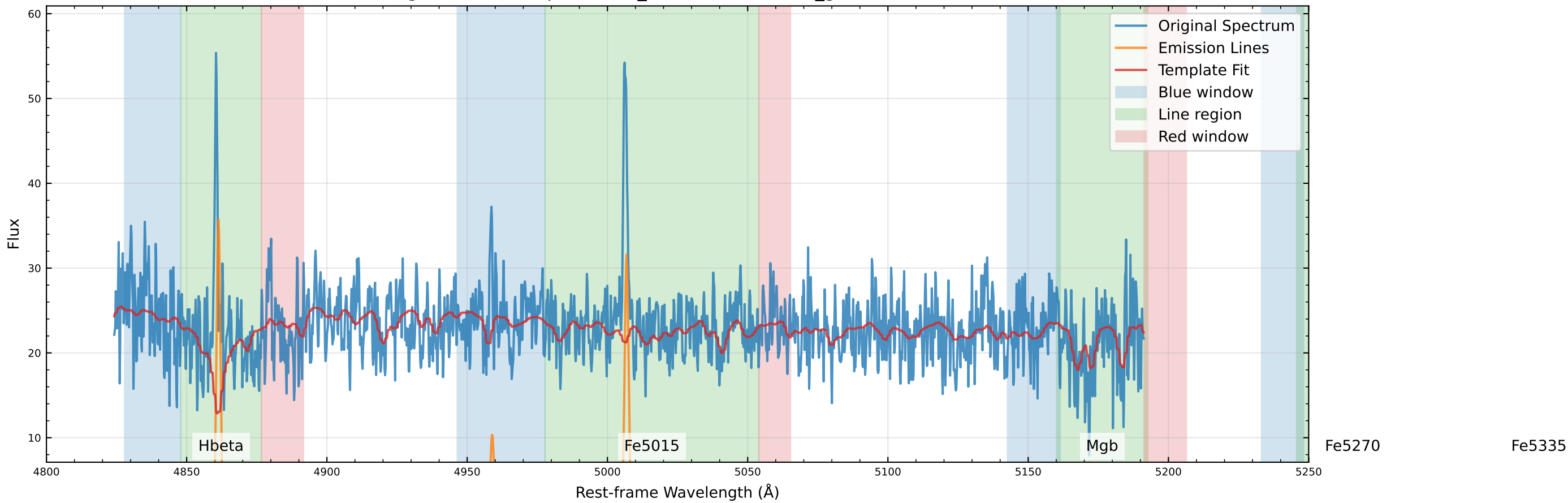
Original Data Comparison (v_star=-35.1 km/s, v_gas=-41.7 km/s)
