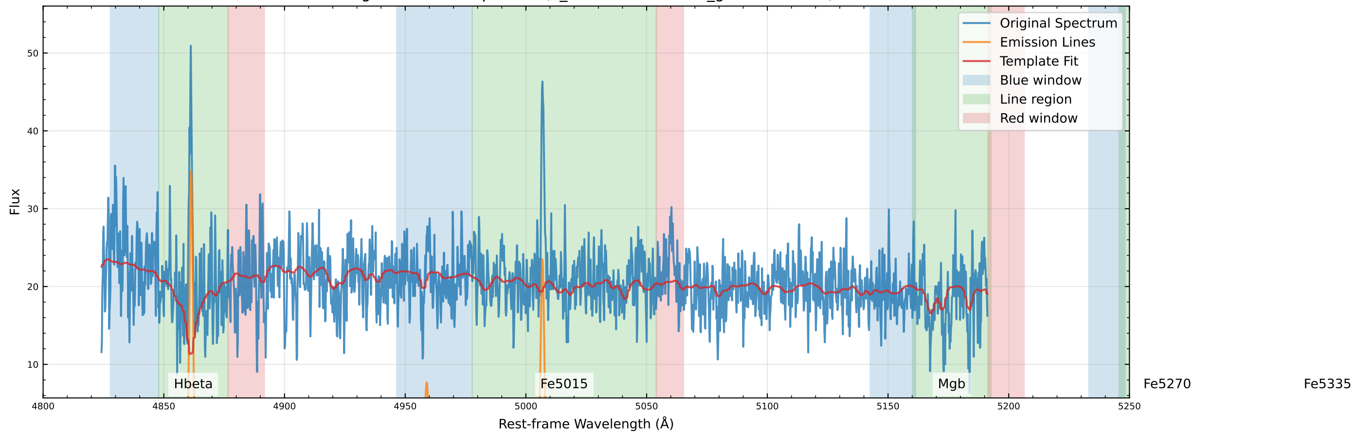
Original Data Comparison ( v_{\text{star}}=21.6 km/s, v_{\text{gas}}=-3.3 km/s)
