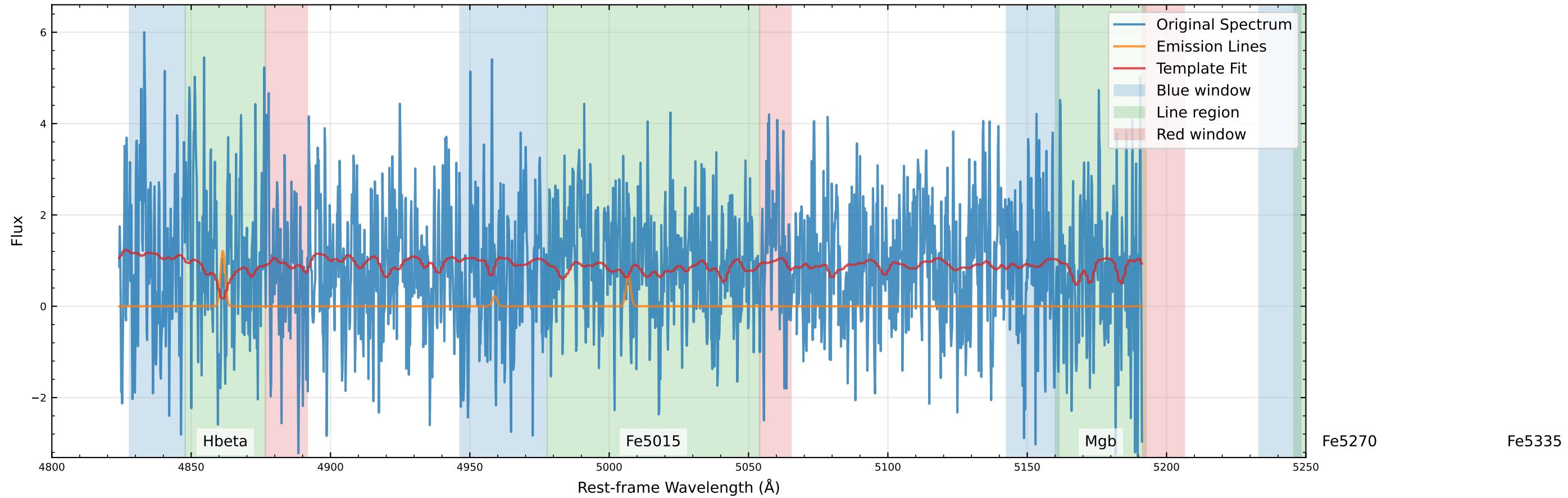
Original Data Comparison (v_star=-218.6 km/s, v_gas=-219.4 km/s)
