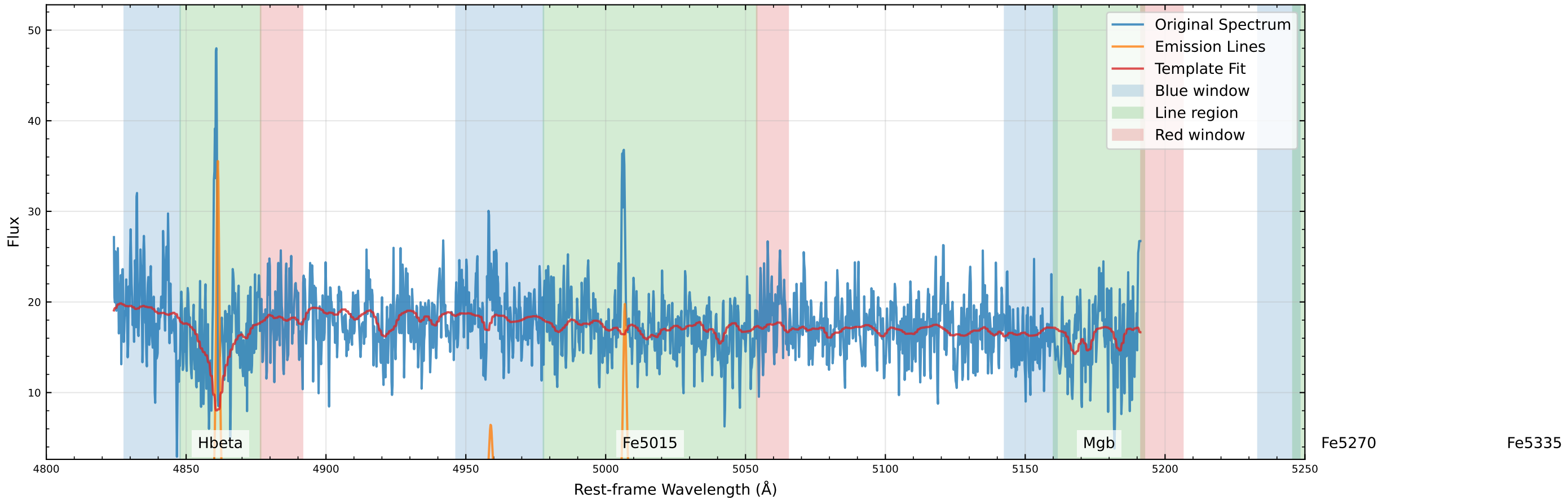
Original Data Comparison (v_star=-38.3 km/s, v_gas=-47.6 km/s)
