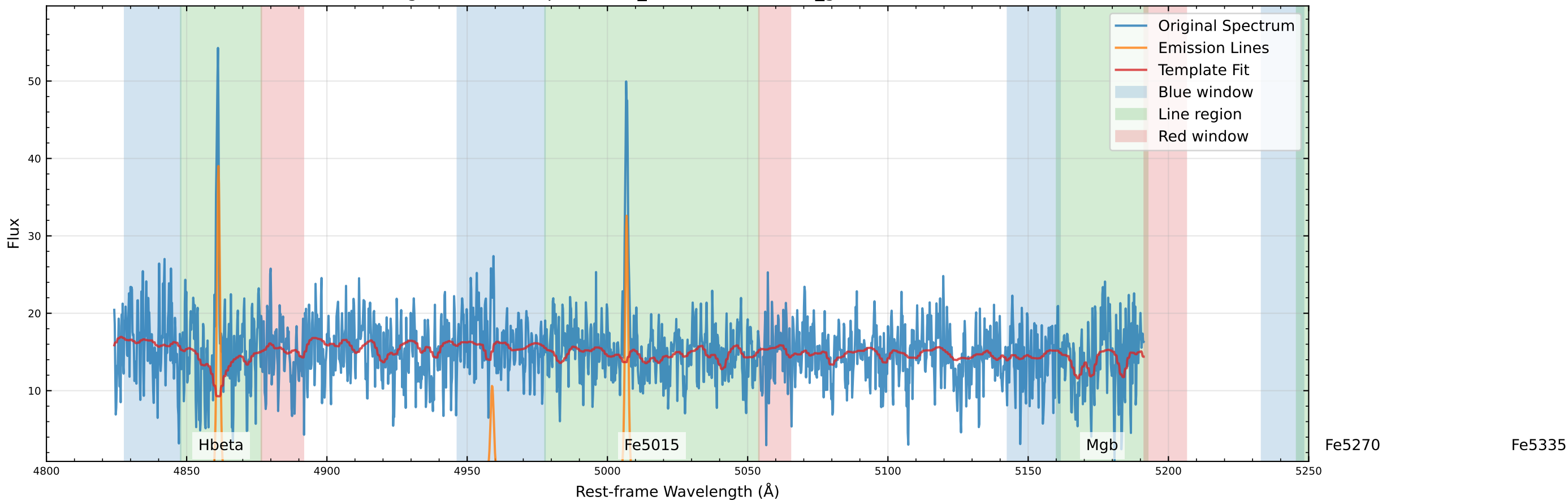
Original Data Comparison (v_star=-15.7 km/s, v_gas=-12.2 km/s)
