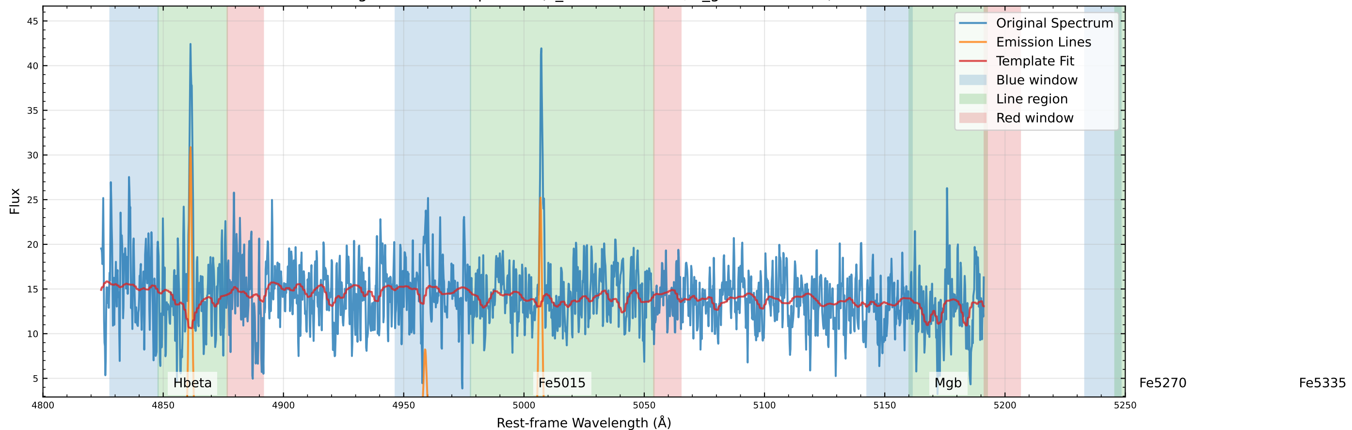
Original Data Comparison (v_star=42.0 km/s, v_gas=17.8 km/s)
