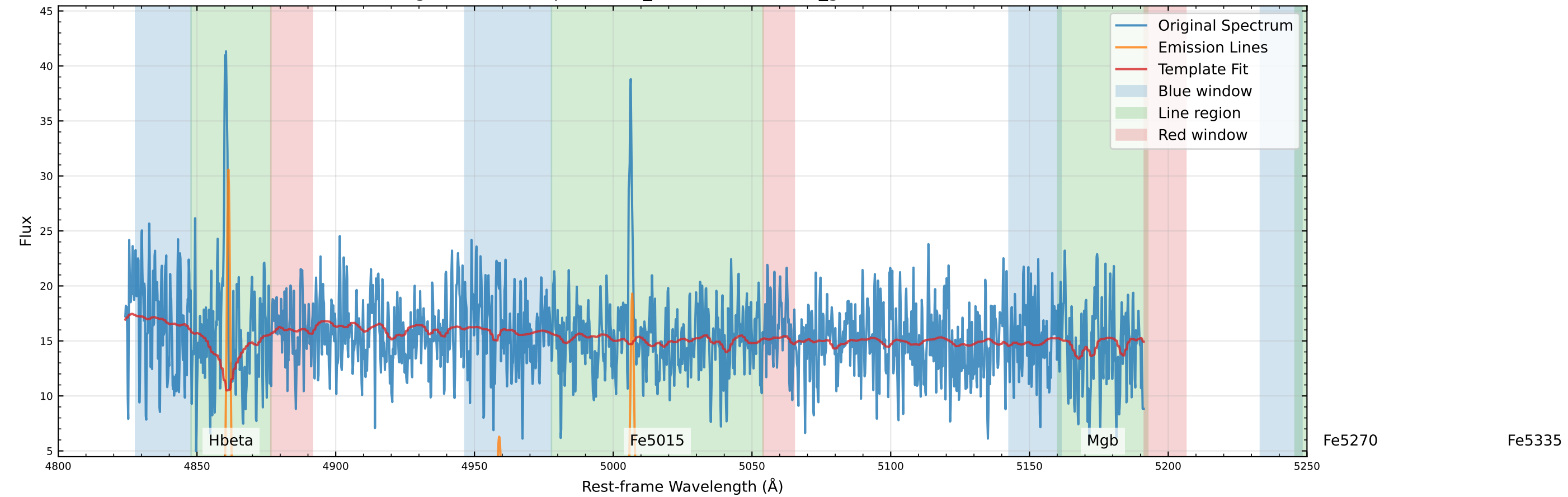
Original Data Comparison (v_star=-59.8 km/s, v_gas=-50.3 km/s)
