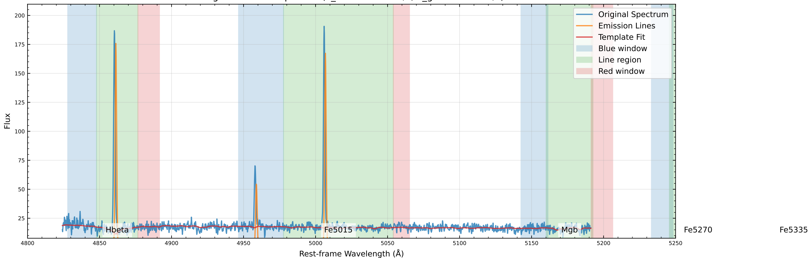
Original Data Comparison (v_star=-38.1 km/s, v_gas=-57.3 km/s)
