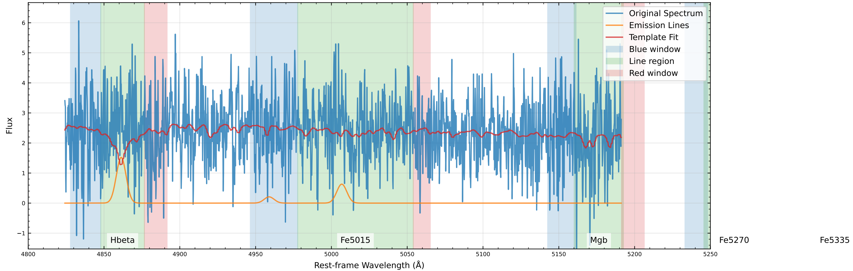
Original Data Comparison (v_star=-175.6 km/s, v_gas=-123.1 km/s)
