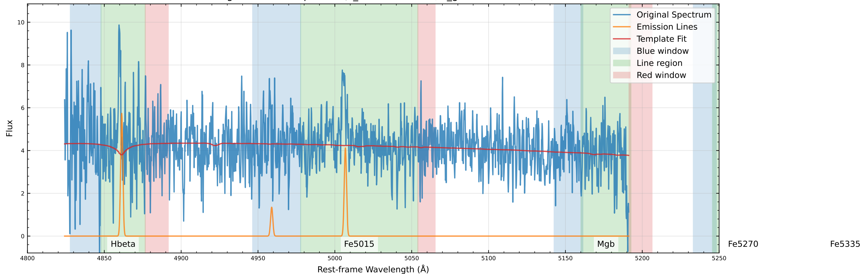
Original Data Comparison (v_star=46.3 km/s, v_gas=-87.0 km/s)
