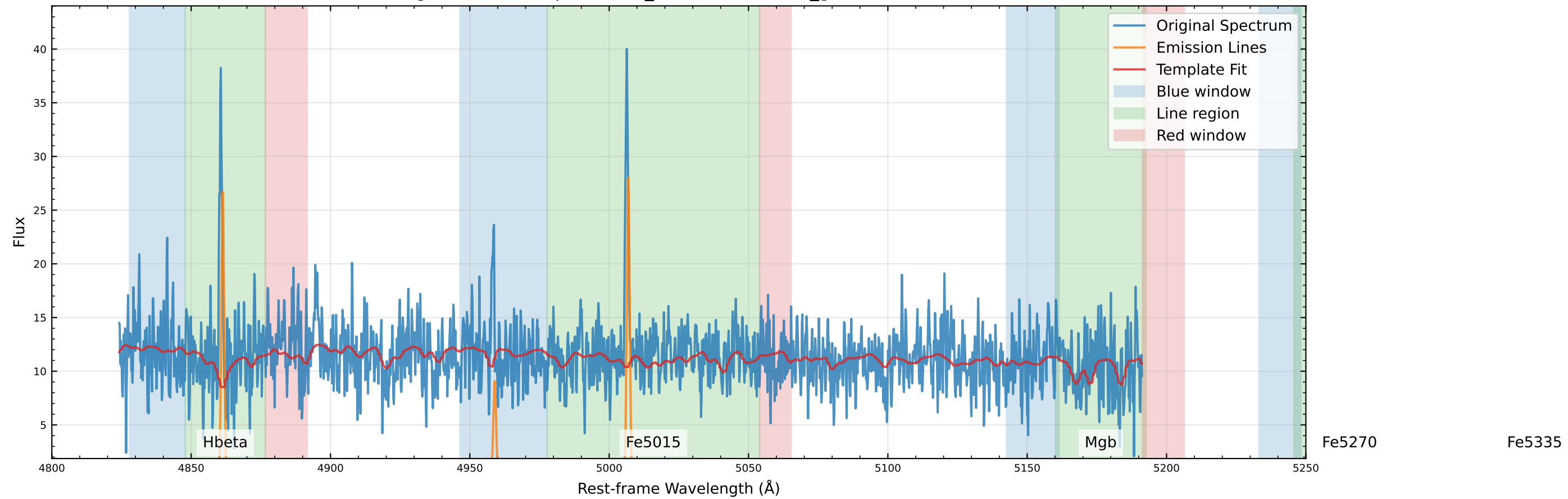
Original Data Comparison (v_star=-7.5 km/s, v_gas=-38.0 km/s)
