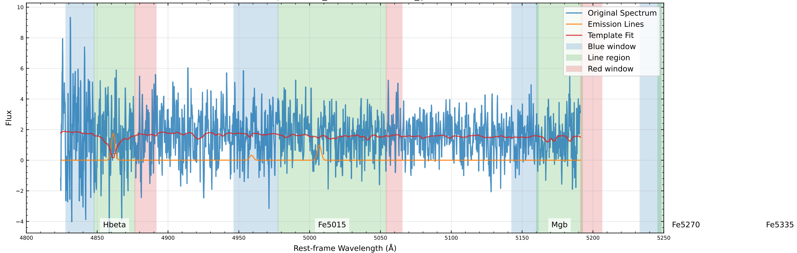
Original Data Comparison (v_star=160.2 km/s, v_gas=140.4 km/s)
