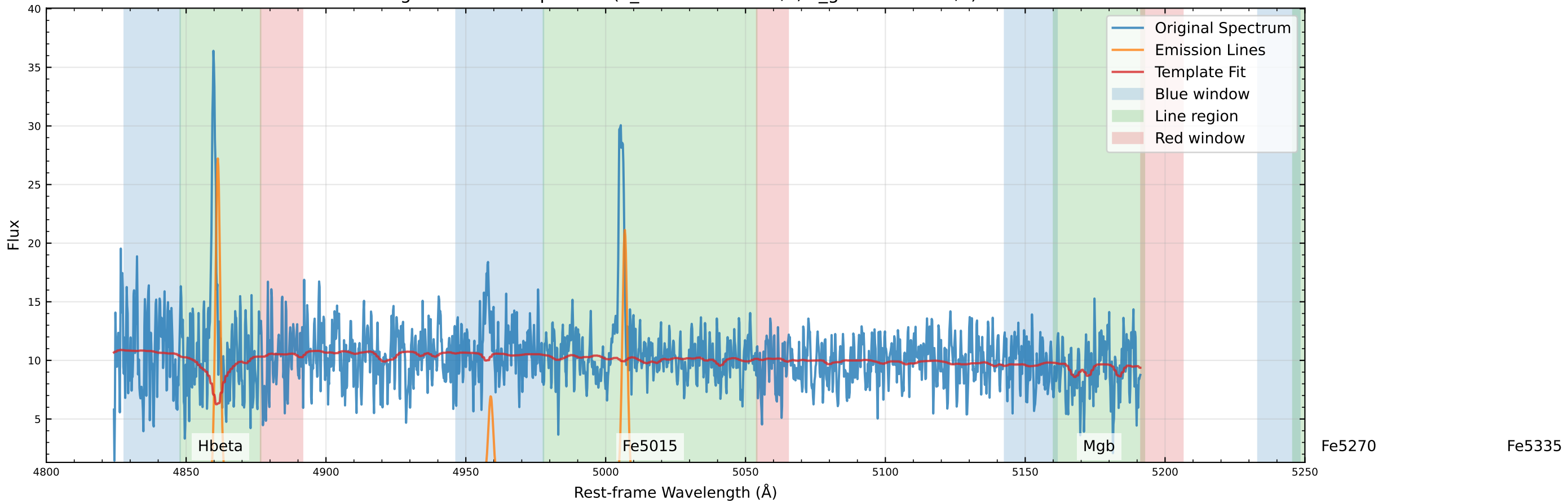
Original Data Comparison (v_star=-100.7 km/s, v_gas=-85.6 km/s)
