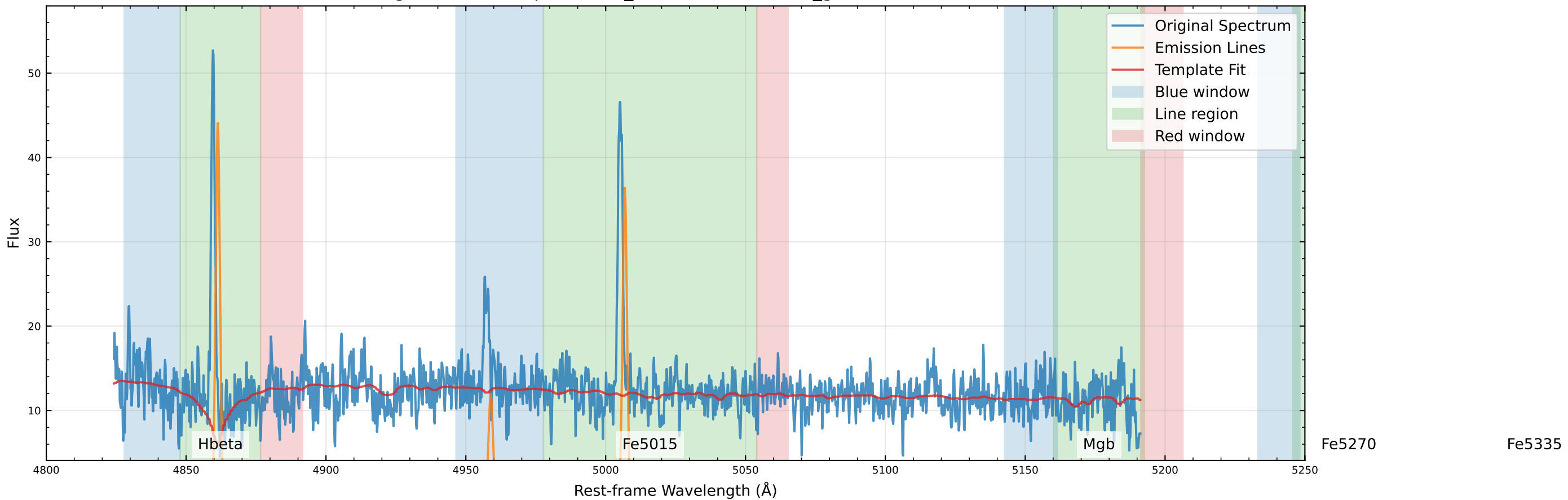
Original Data Comparison (v_star=-107.3 km/s, v_gas=-102.1 km/s)
