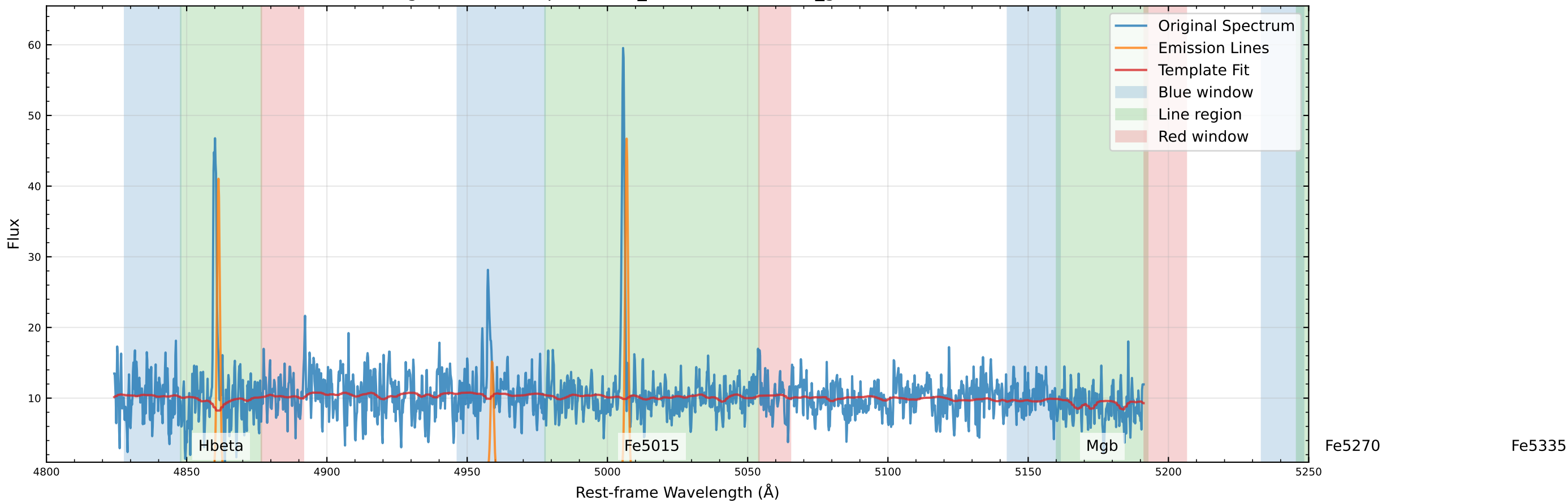
Original Data Comparison (v_star=-69.0 km/s, v_gas=-75.1 km/s)
