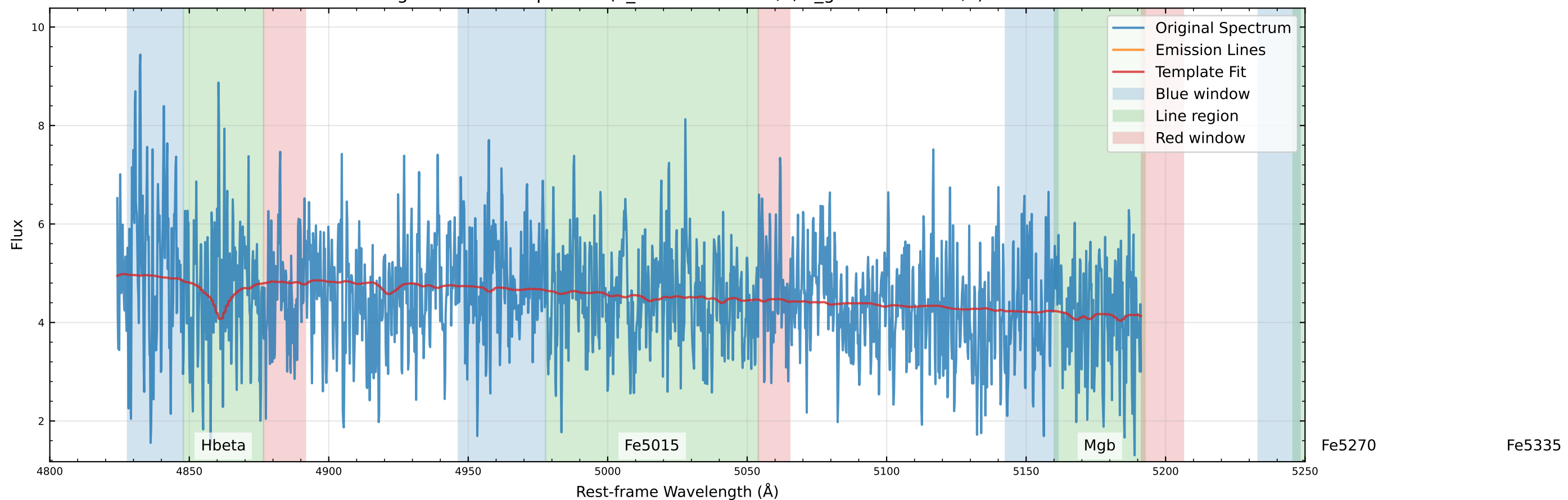
Original Data Comparison (v_star=-260.0 km/s, v_gas=-259.9 km/s)
