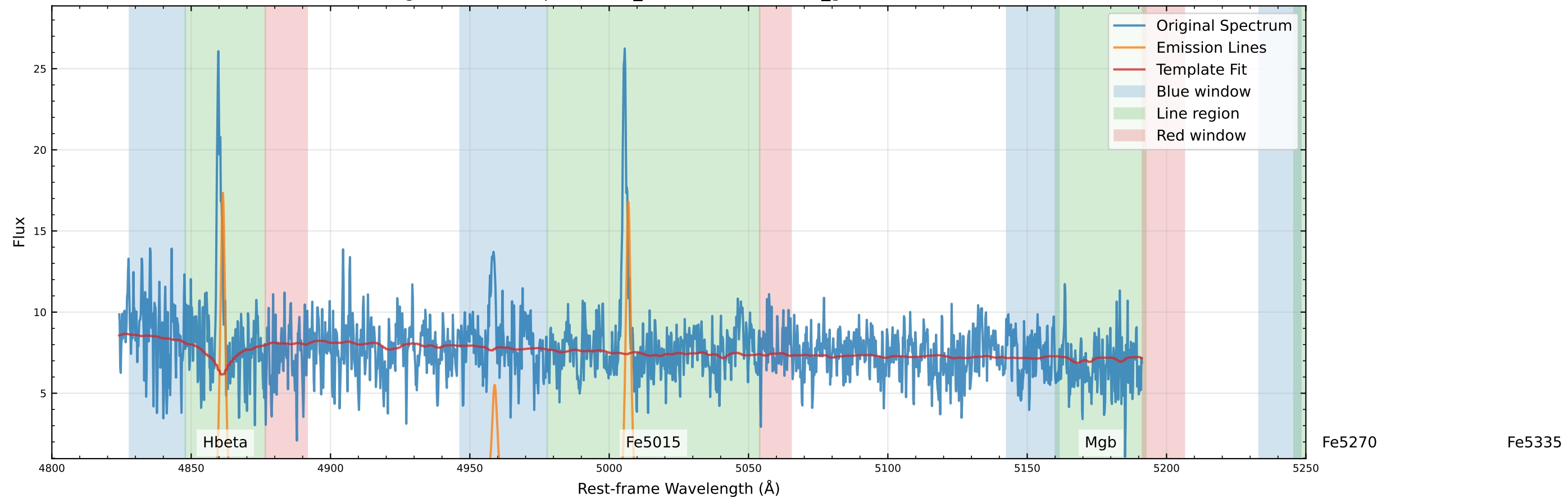
Original Data Comparison (v_star=-101.6 km/s, v_gas=-78.2 km/s)
