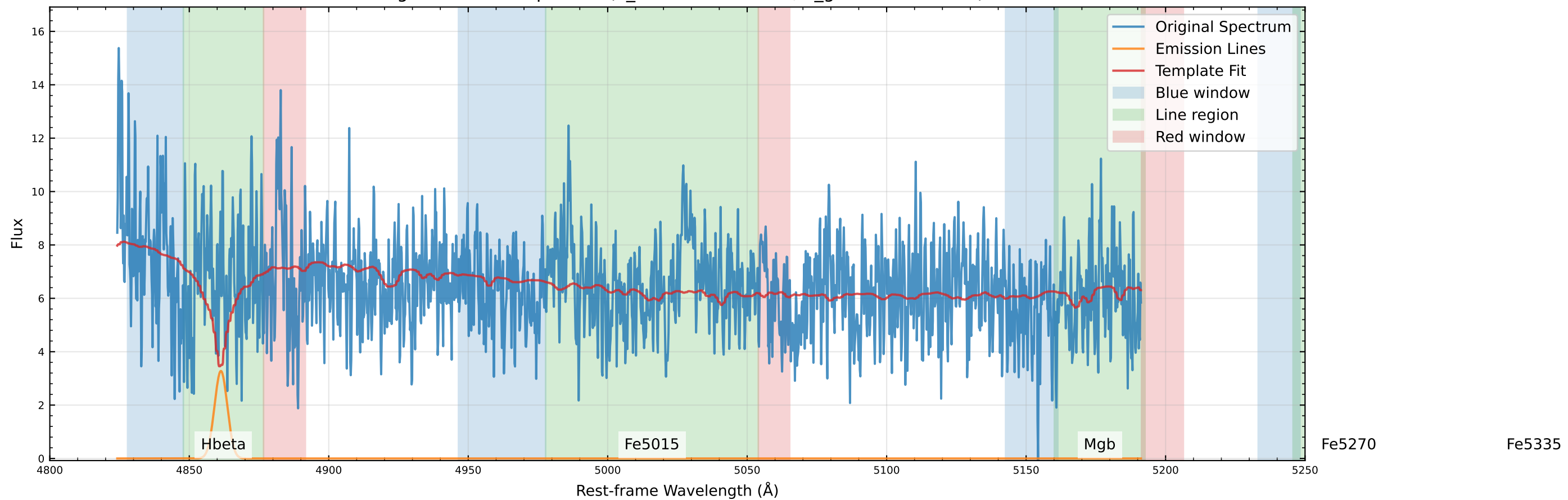
Original Data Comparison (v_star=-277.5 km/s, v_gas=-372.6 km/s)
