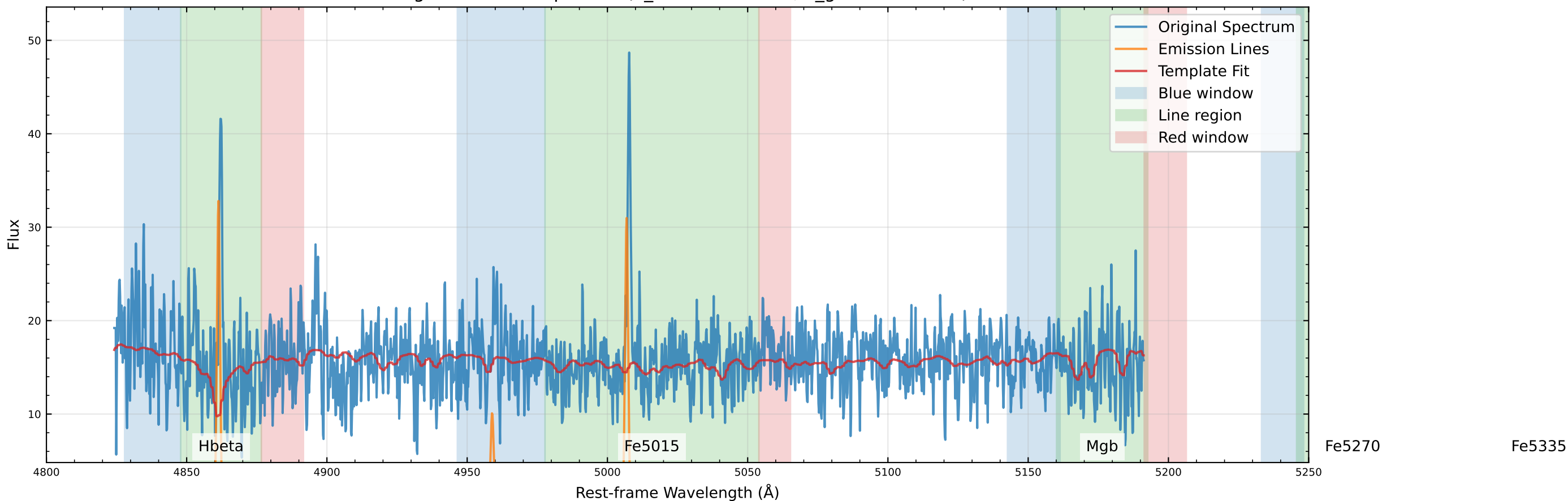
Original Data Comparison (v_star=76.0 km/s, v_gas=51.6 km/s)
