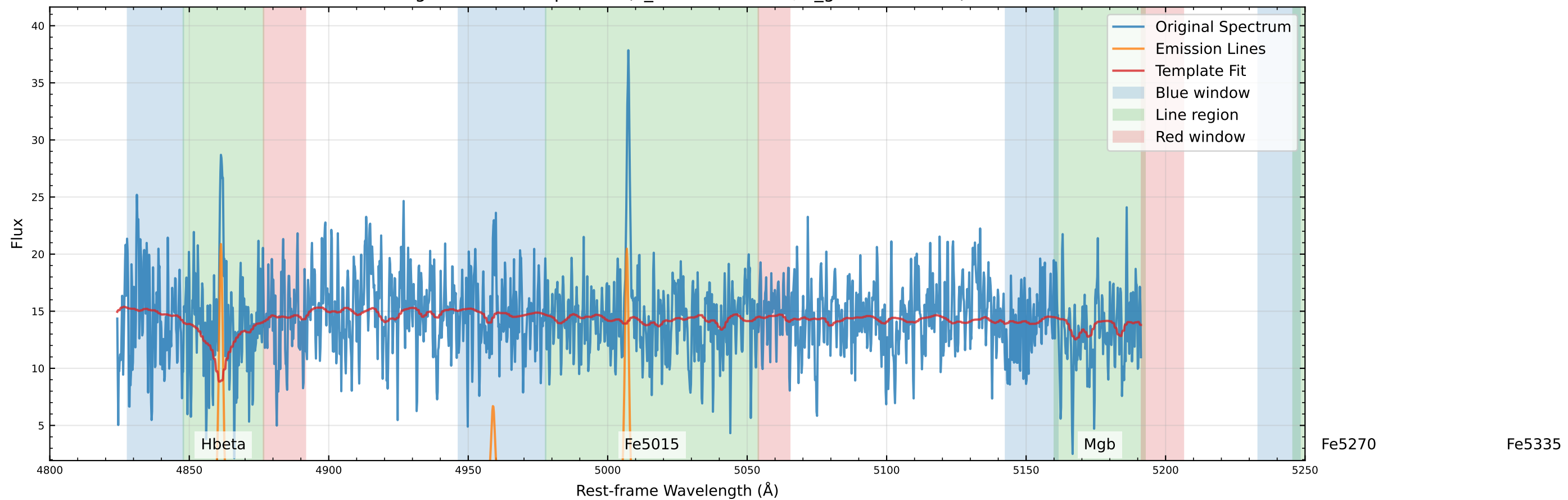
Original Data Comparison (v_star=10.9 km/s, v_gas=25.6 km/s)
