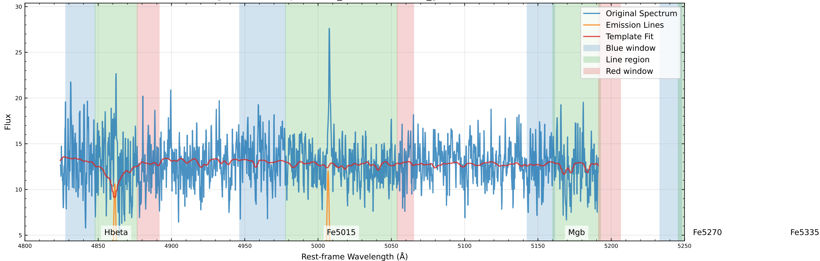
Original Data Comparison (v_star=59.8 km/s, v_gas=47.0 km/s)
