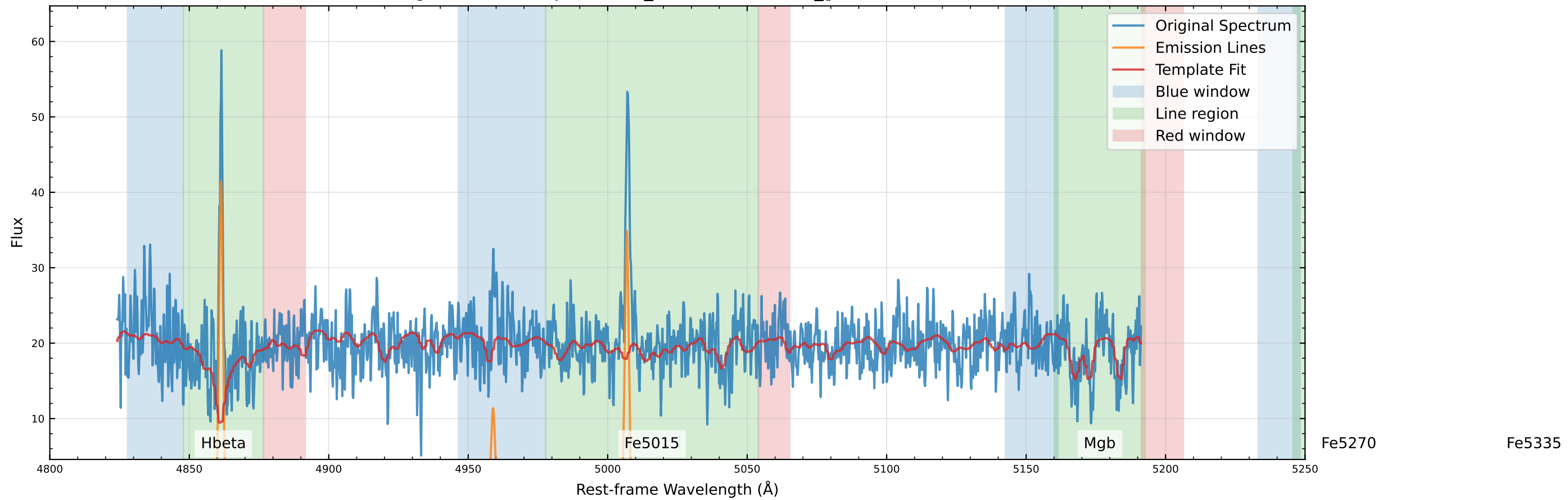
Original Data Comparison (v_star=32.4 km/s, v_gas=11.7 km/s)
