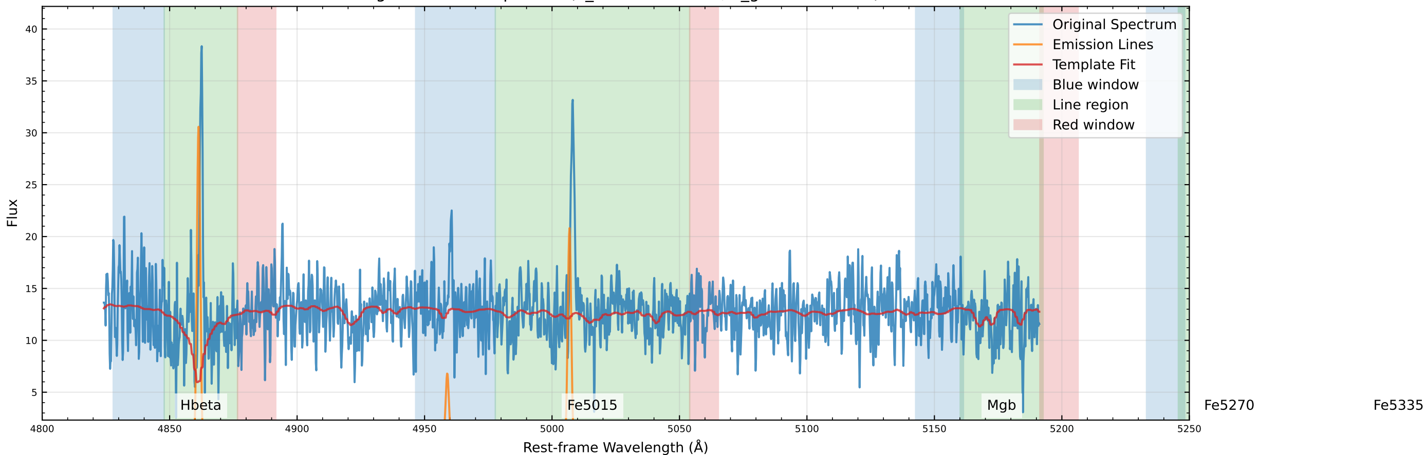
Original Data Comparison (v_star=37.2 km/s, v_gas=66.8 km/s)
