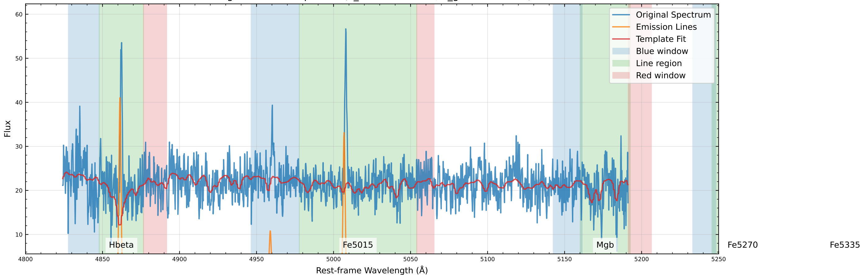
Original Data Comparison (v_star=39.8 km/s, v_gas=58.1 km/s)
