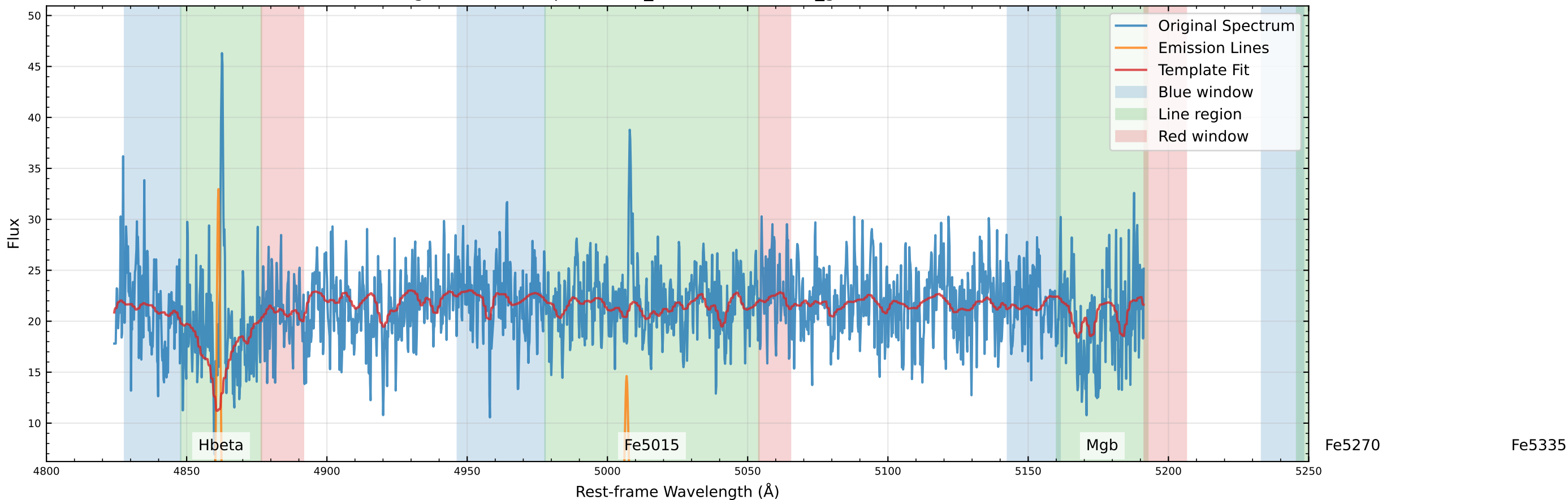
Original Data Comparison (v_star=70.6 km/s, v_gas=78.9 km/s)
