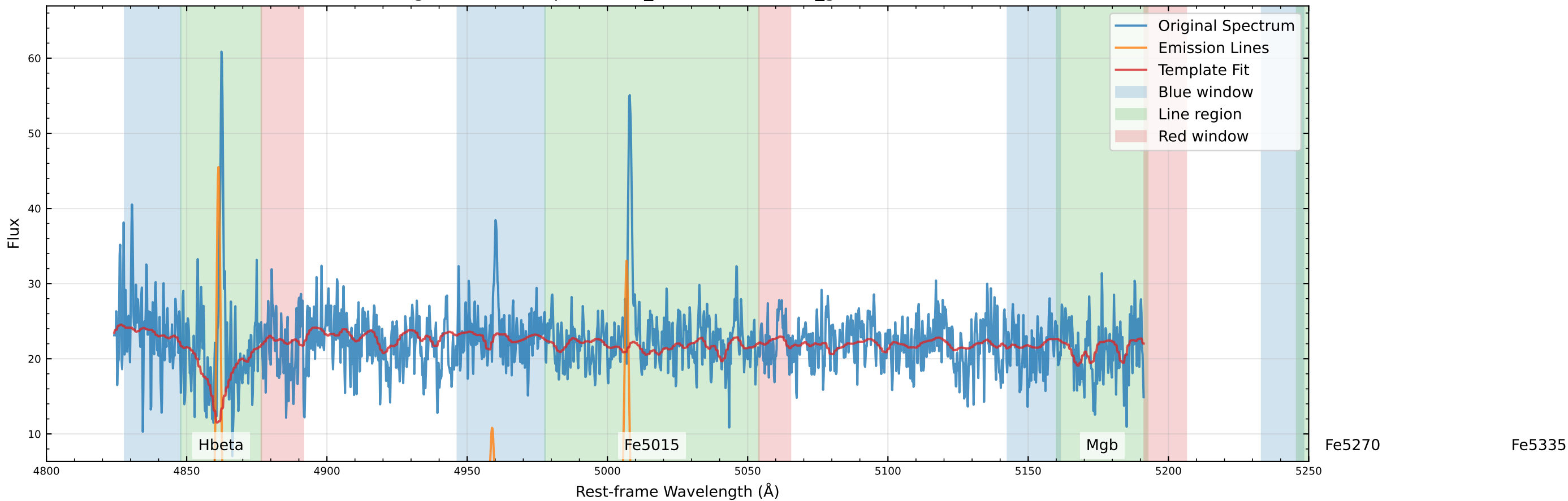
Original Data Comparison (v_star=63.5 km/s, v_gas=71.0 km/s)
