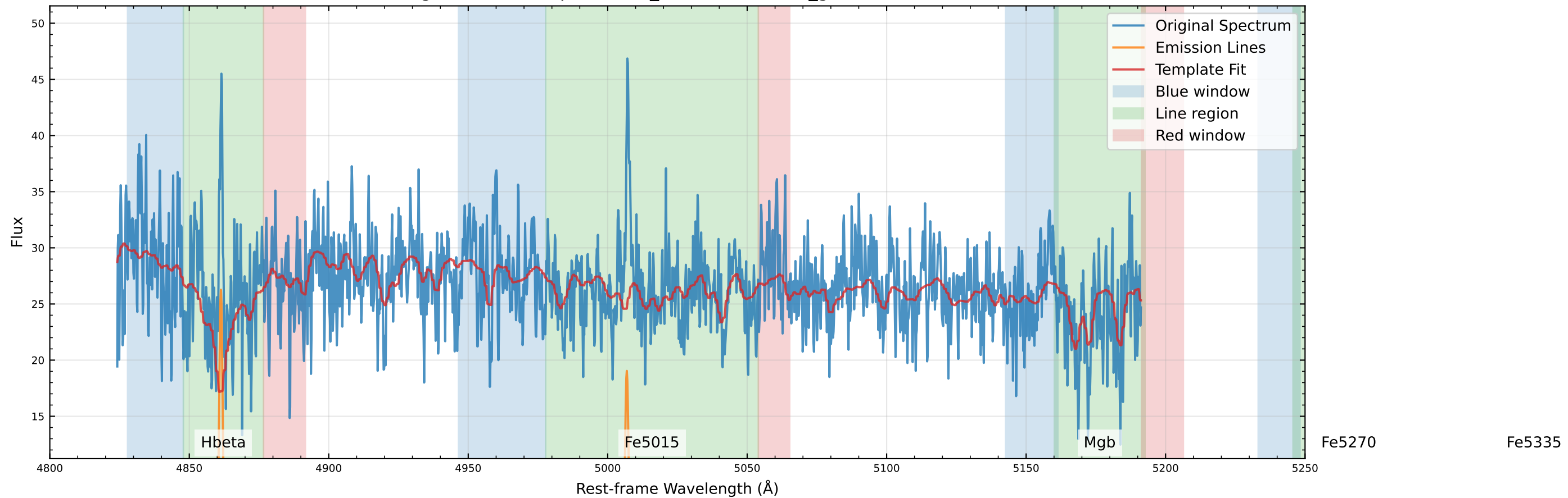
Original Data Comparison (v_star=3.0 km/s, v_gas=11.2 km/s)
