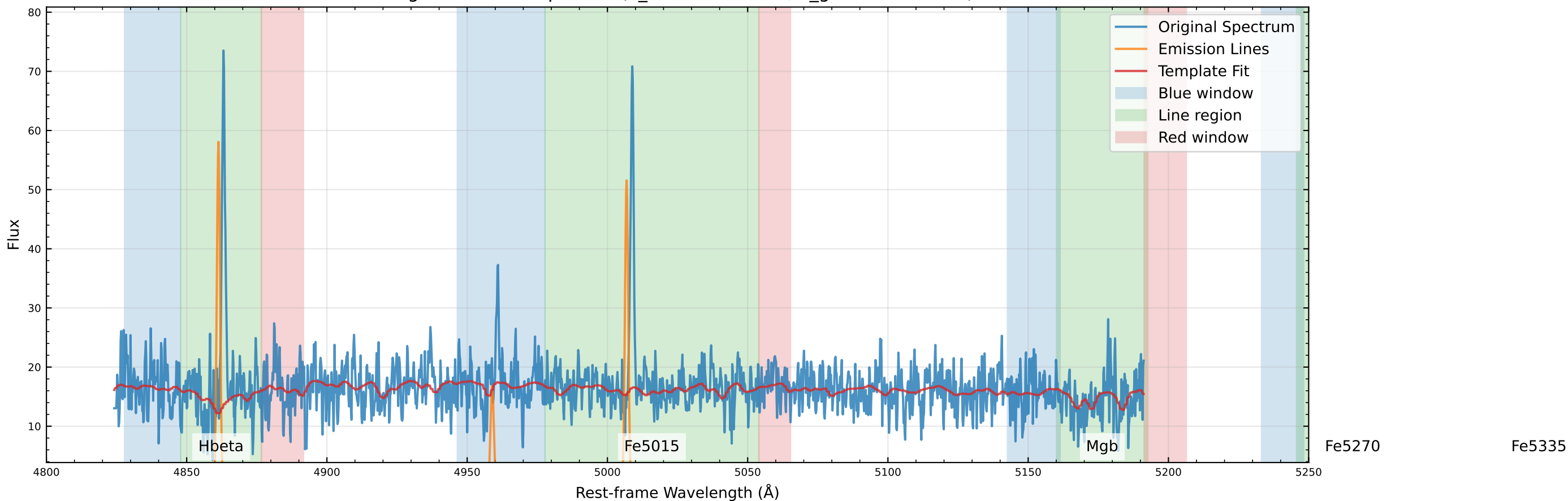
Original Data Comparison (v_star=89.1 km/s, v_gas=114.1 km/s)
