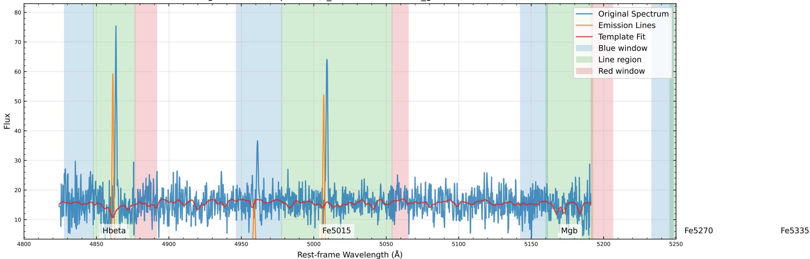
Original Data Comparison (v_star=129.2 km/s, v_gas=132.6 km/s)
