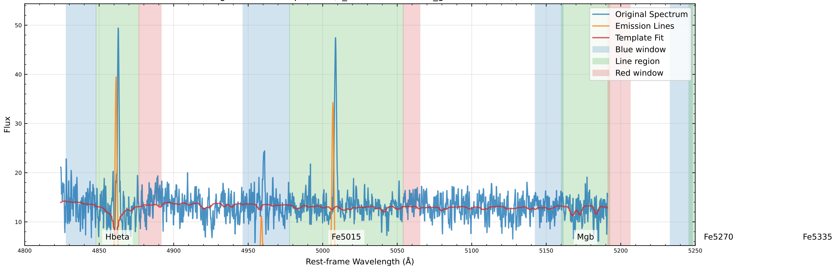
Original Data Comparison (v_star=78.9 km/s, v_gas=97.0 km/s)
