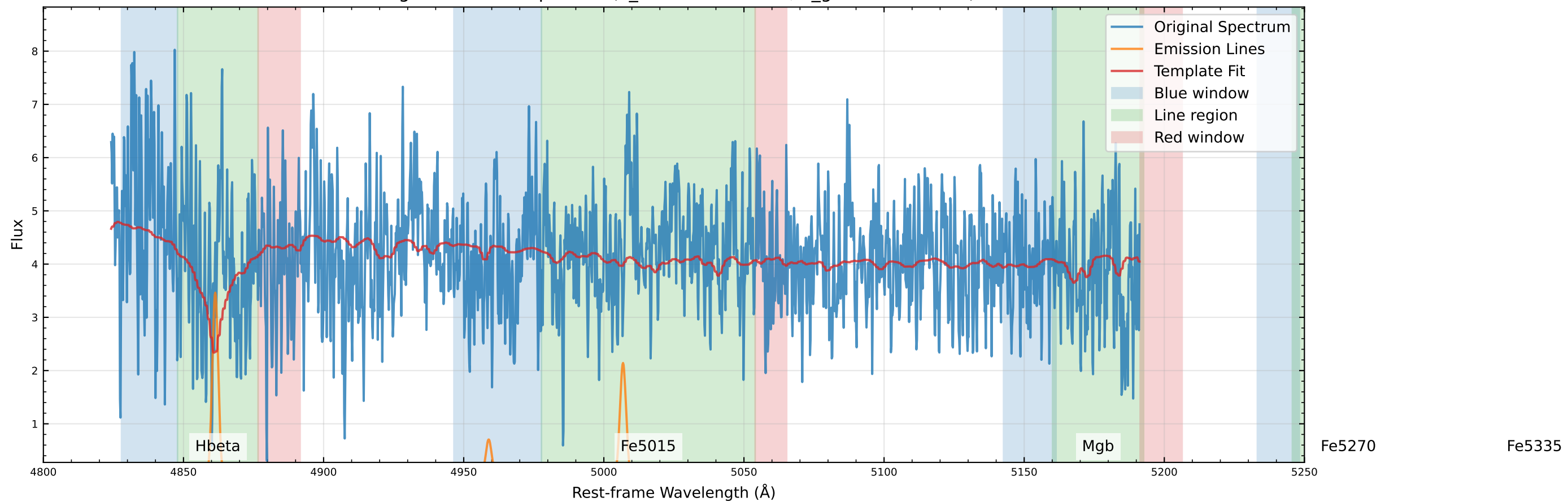
Original Data Comparison (v_star=109.0 km/s, v_gas=121.4 km/s)
