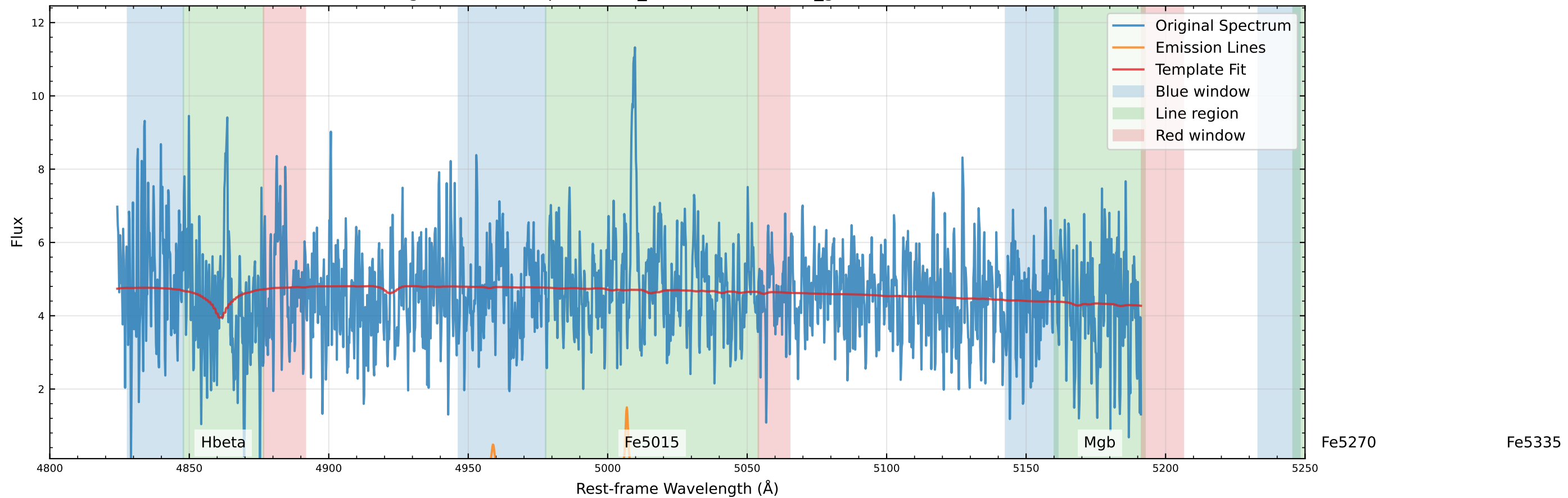
Original Data Comparison ( v_{\text{star}}=-39.3 km/s, v_{\text{gas}}=-46.6 km/s)
