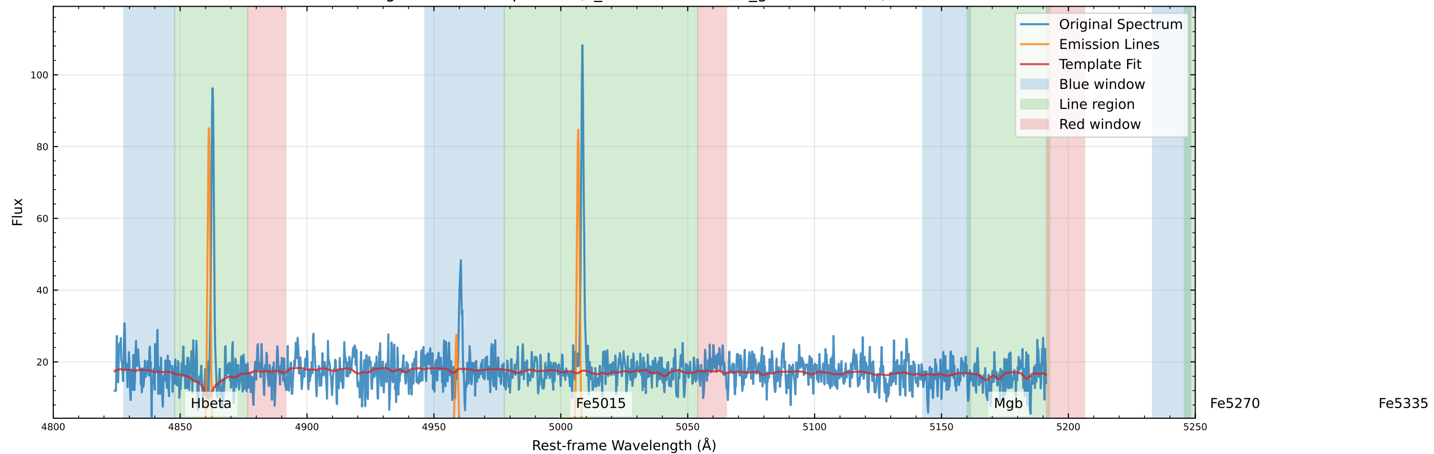
Original Data Comparison (v_star=69.2 km/s, v_gas=95.2 km/s)
