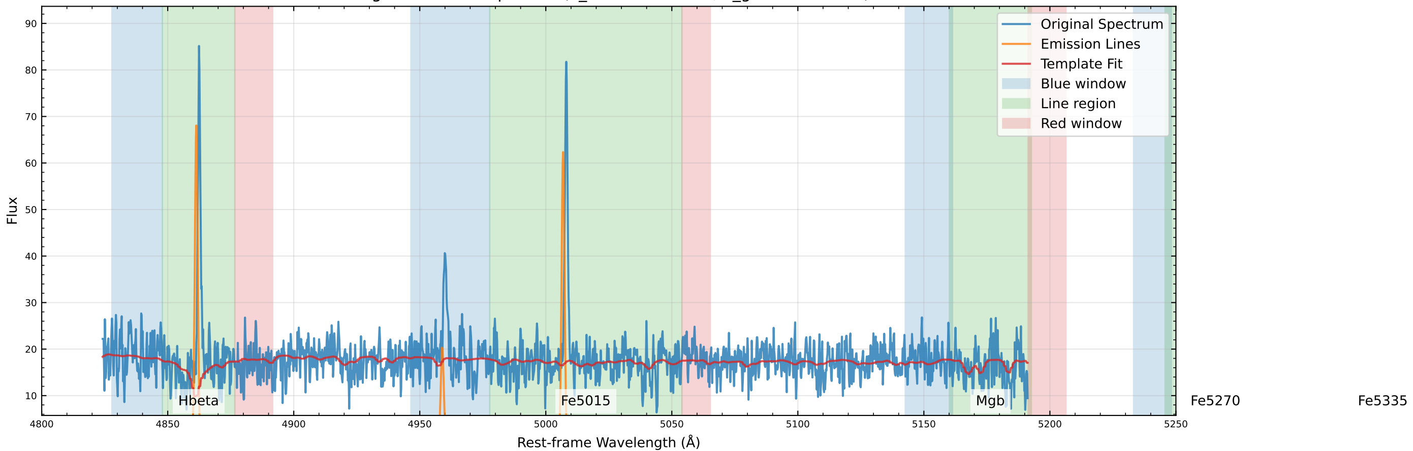
Original Data Comparison (v_star=49.4 km/s, v_gas=72.7 km/s)
