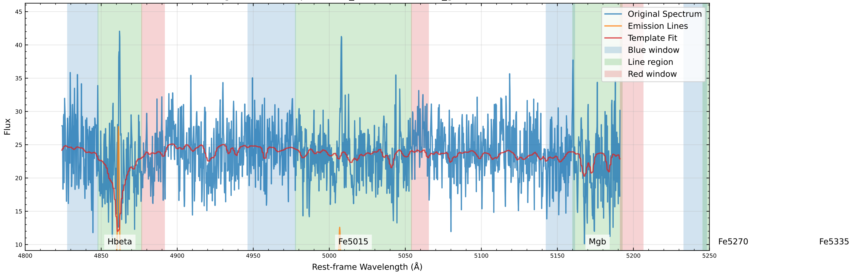
Original Data Comparison (v_star=40.8 km/s, v_gas=47.4 km/s)
