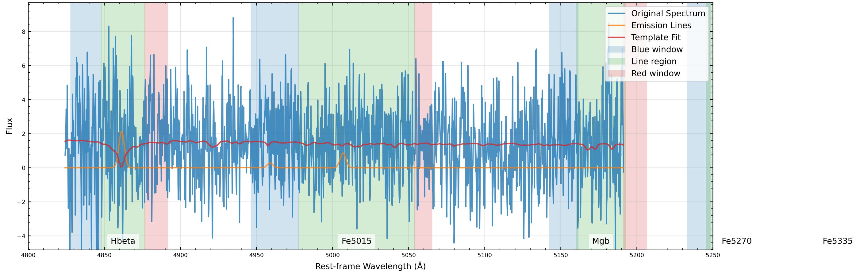
Original Data Comparison (v_star=167.4 km/s, v_gas=319.9 km/s)
