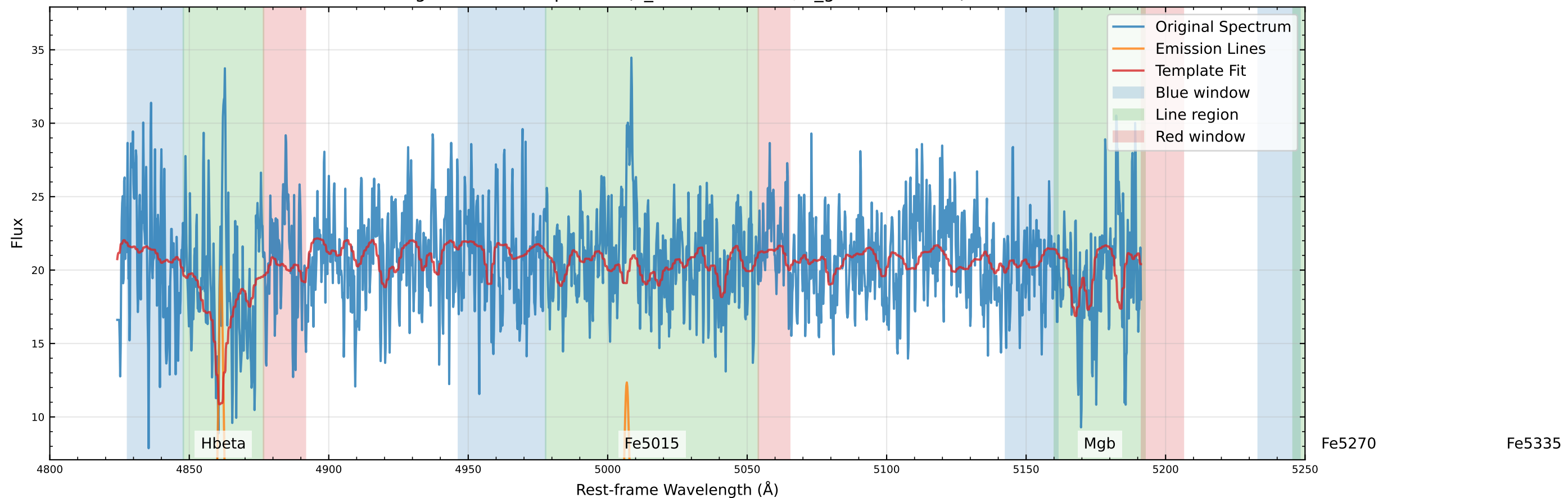
Original Data Comparison (v_star=87.6 km/s, v_gas=73.5 km/s)
